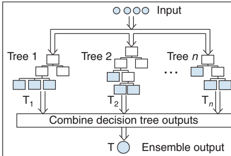
Figure 4. Schematic framework of the ensemble tree model presented by Weng and Meng (2012)
