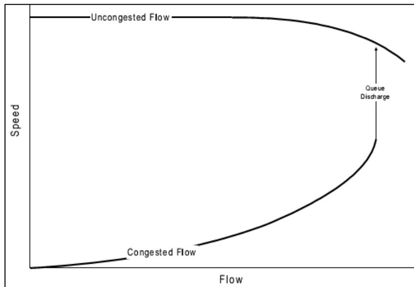
Figure 19. Traffic speed-flow relationship ( HCM, 2010 )
