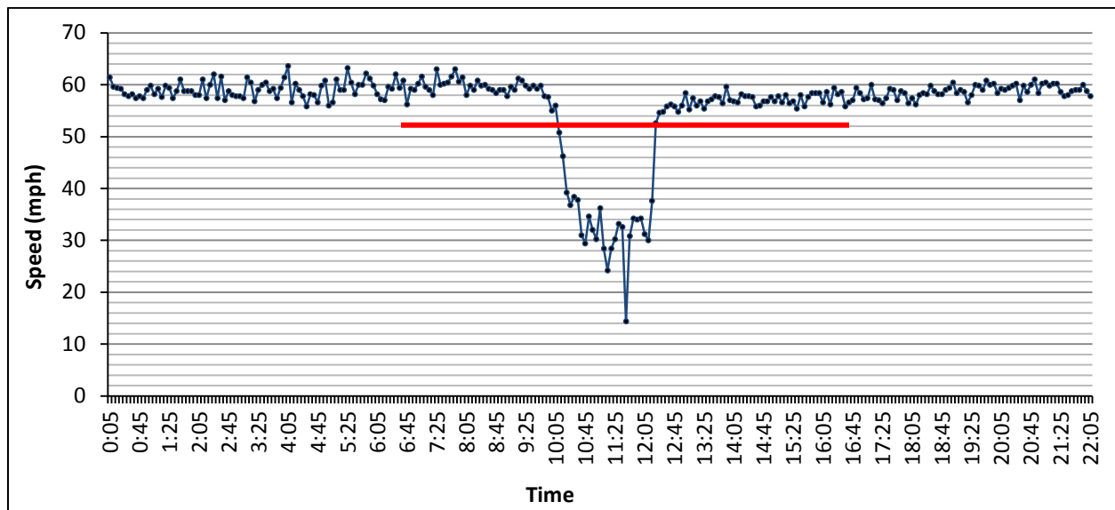
Figure 18. Speed-time graph to determine the time of the breakdown for the Equation (7)
