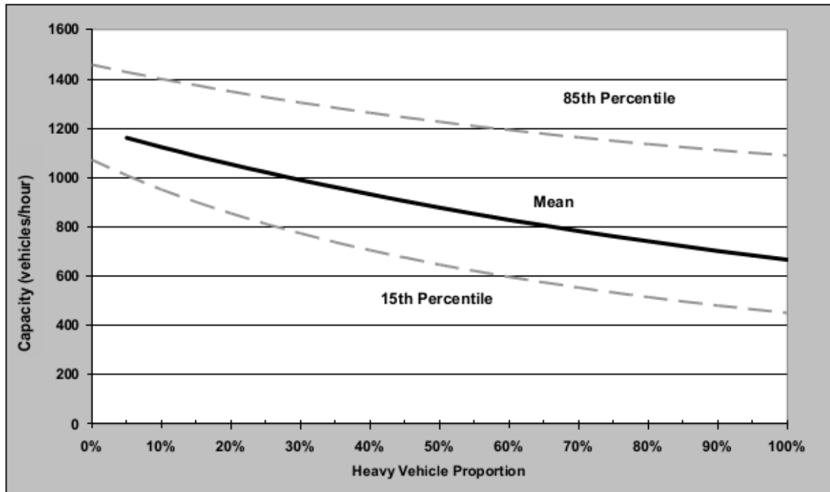
Figure 2. Variation in capacity vs. heavy vehicle percentage ( Pringle et al., 2010 )
