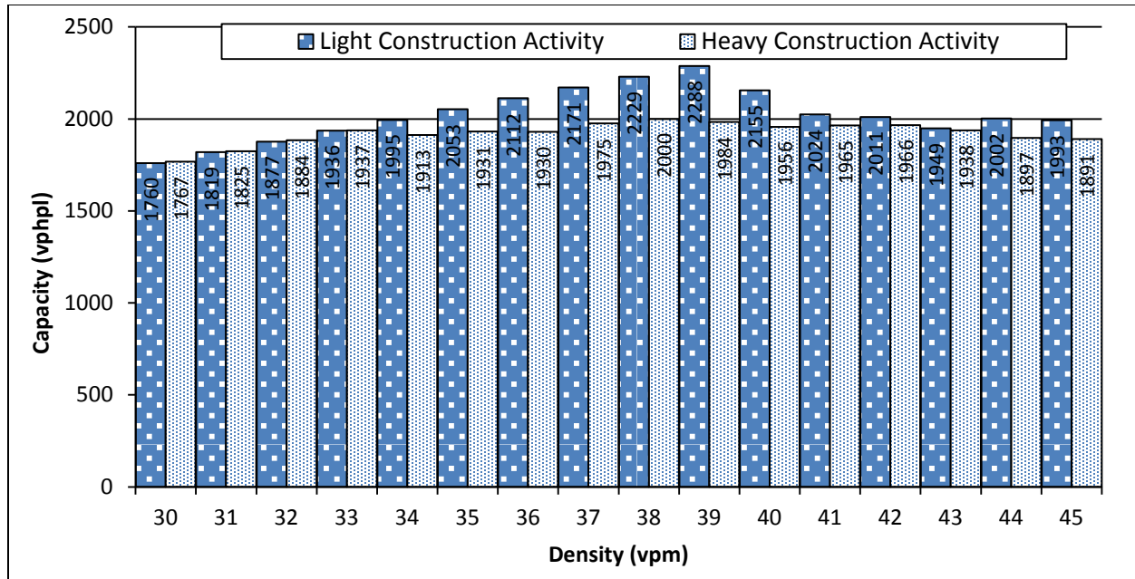
Figure 31. Capacity values, all days combined for each construction activities
