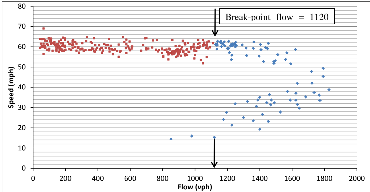
Figure 22. Determining the break-point flow in the speed-flow graph
