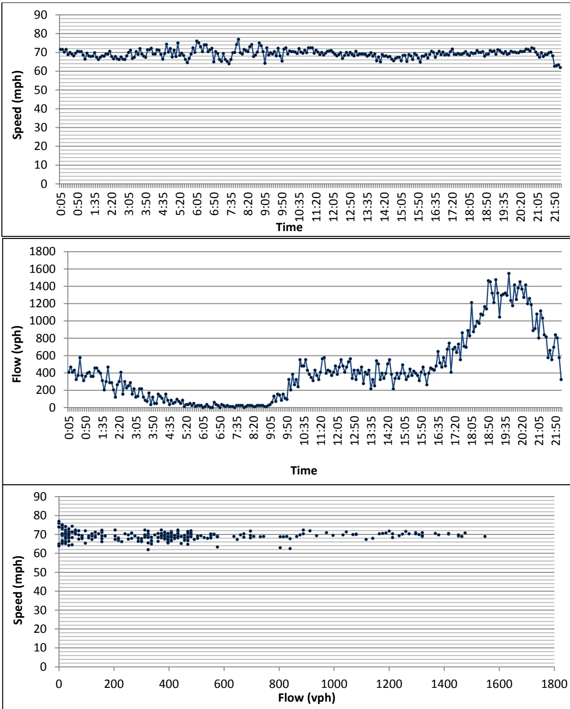
Figure 15. Graphs of speed-time (top), flow-time (middle), and speed-flow (bottom) for lane 3 of the westbound direction at mile marker 267.4 on August 28, 2012
